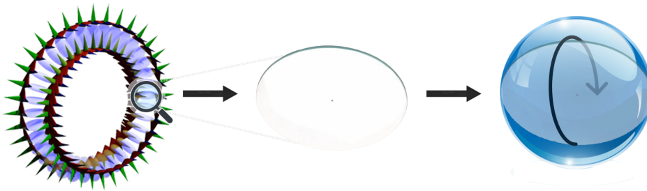
Fig. 3.6: Each lens represents a diameter slice of the electron's overall spherical charge field
