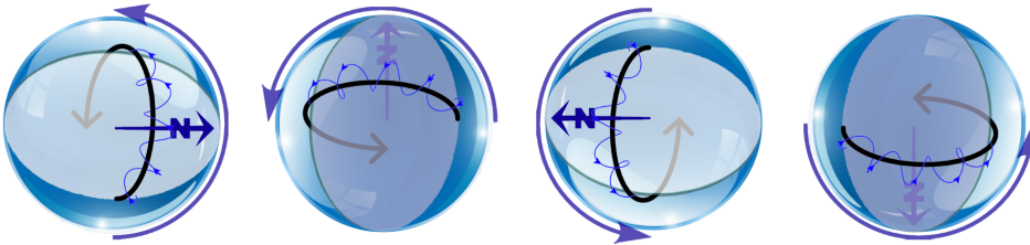
Fig. 4.6: Sequence showing the tumble of an electron made of a left circularly-polarised photon
