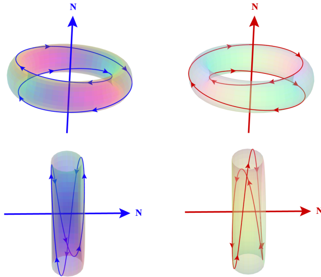
Fig. 4.1: Electrons with a left -circularly-polarised photon (left) and a right -circularly-polarised photon (right).
