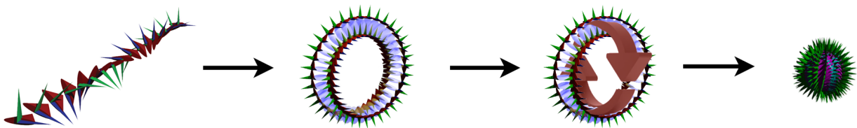
Fig. 3.5: The angular momentum consequences of a right-circularly-polarized photon forming a light-speed, double-loop rotation.
